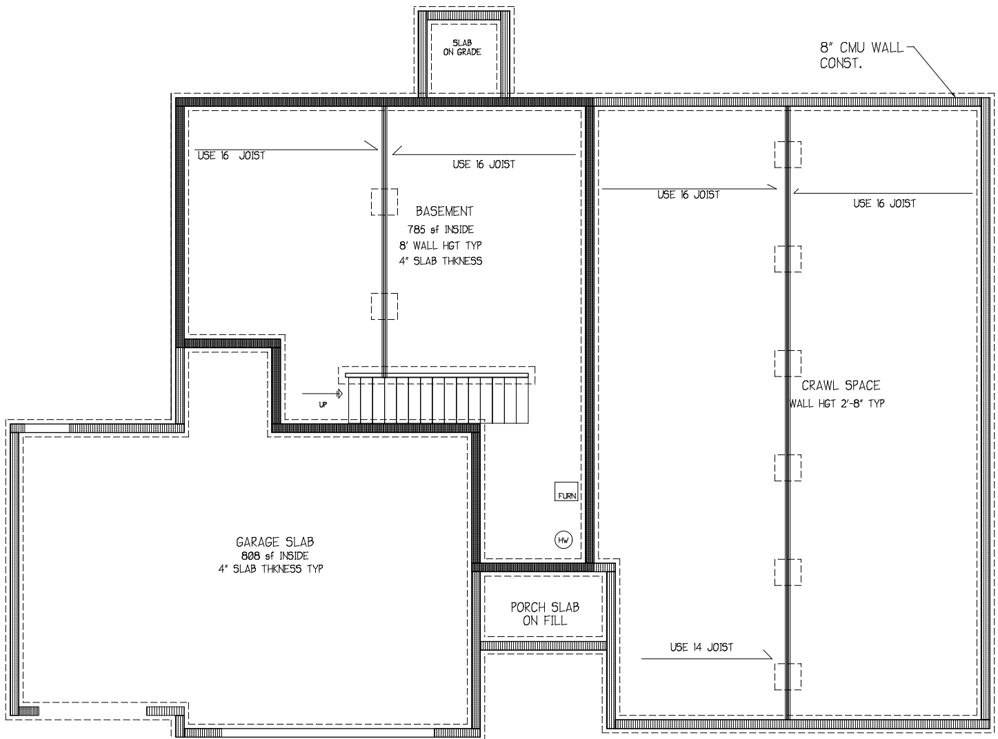
INVERNESS MODEL FOUNDATION PLAN
